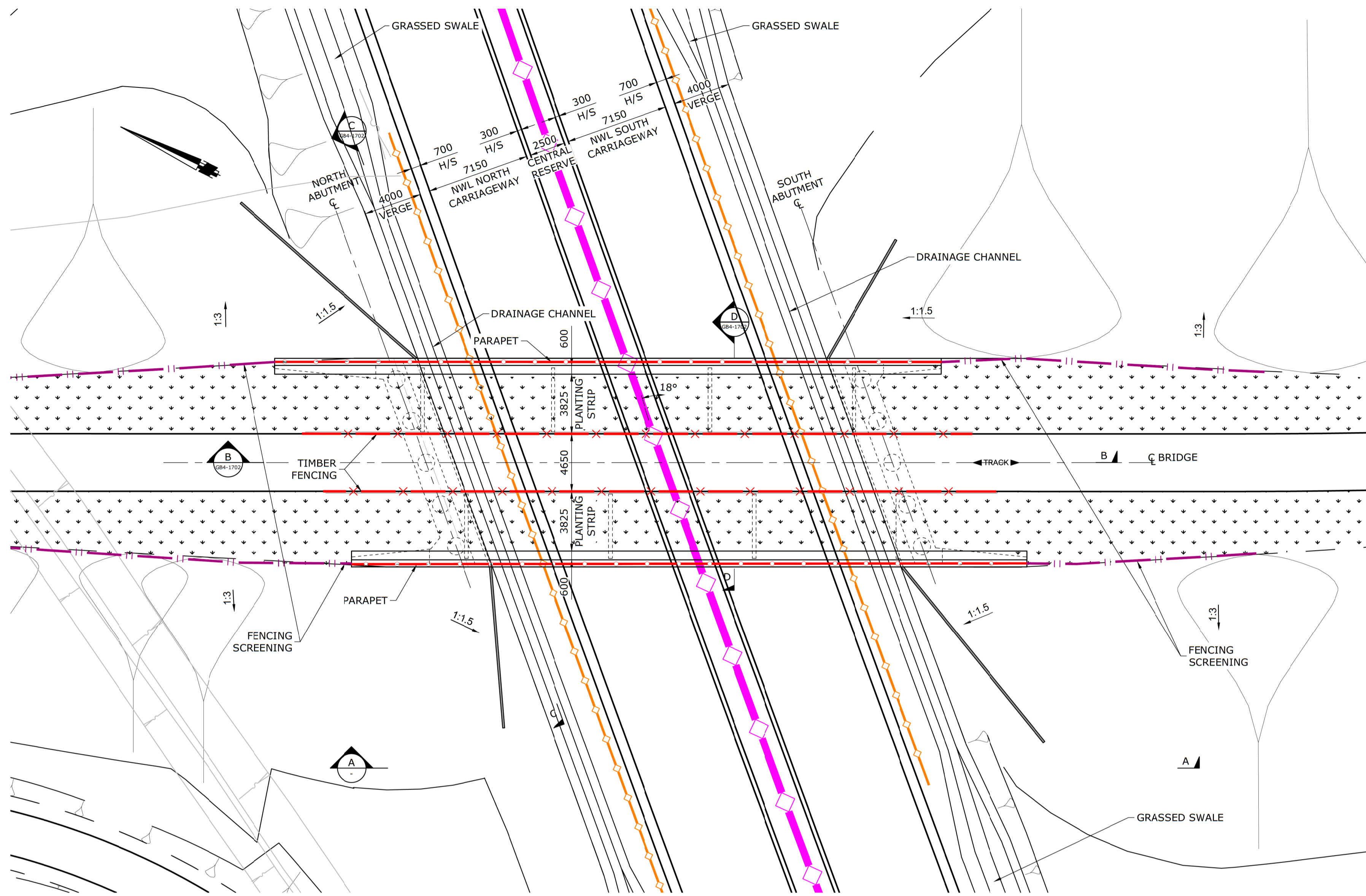
PLAN 1:200
